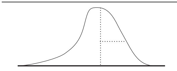
Figure 5.5. Nonsymmetrical Distribution with Fat Tail
